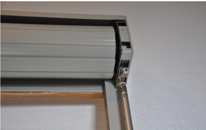
7. Temporarily attach crank to install slat
